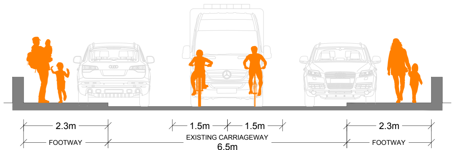
TYPICAL CROSS SECTION Esc 1:50
